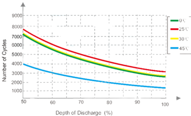
Different DOD Discharge and Different Temperature Cycle Life Curve @0.2C 25C
